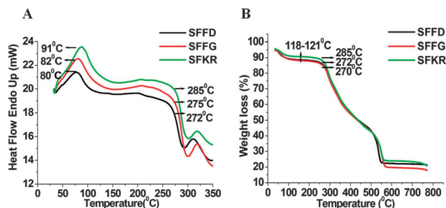
Fig. 2 (A and B) Differential scanning calorimetry (DSC) and thermo-gravimetric analysis (TGA) of pure SF and SFKR blended 3D scaffolds.
