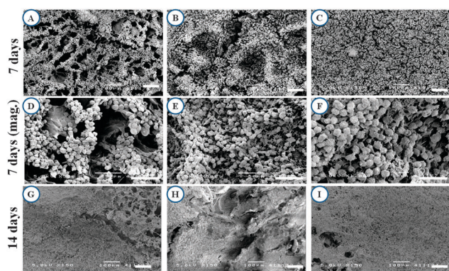
Fig. 6 SEM pictographs of constructs, after 7 days and 14 days of cell culture using L929 (murine fibroblast) on pure SF and SFKR scaffolds. SFFD scaffolds (2%, w/w) (A, D and G), SFFD scaffolds (B, E and H) and SFKR blended scaffolds (2%, w/w) (C, F and I). Scale bar represents 50 and 100 \mu\text{m} , respectively.
